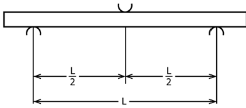
FIG. 1 Loading System for Test Method I
